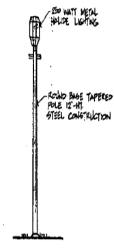
STREET LAMP DETAIL NO SCALE
