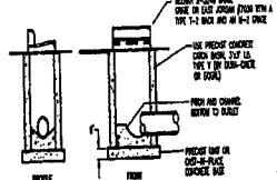
2x3 CURB INLET DETAIL 1/4"=1'-0"
