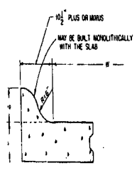
INTEGRAL CONCRETE CURB & GUTTER TYPE II NOT TO SCALE
