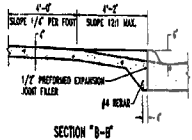
STANDARD HANDICAP RAMPS NOT TO SCALE
