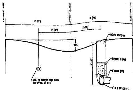
UTILITY LOCATIONS IN TRENCH 1/4"=1'-0"
