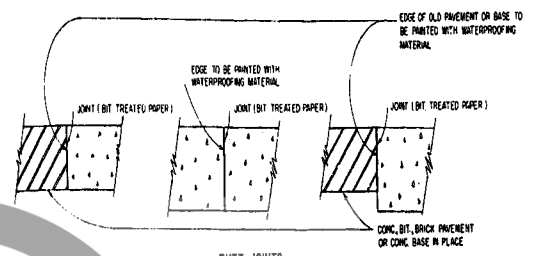
BUTT JOINTS NOT TO SCALE NOTE: IF TRANSVERSE JOINTS IN THE ADJACENT PAVEMENTS ARE IDENTICAL AS TO LOCATION AND TYPE, THE BITUMINOUS TREATED PAPER MAY BE OMITTED, IN WHICH CASE AN ADDITIONAL HEAVY APPLICATION OF WATERPROOFING SHALL BE SUBSTITUTED THEREFOR
