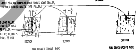
DETAILS OF SEAL FOR PAVEMENT CONTRACTION JOINTS NOT TO SCALE
