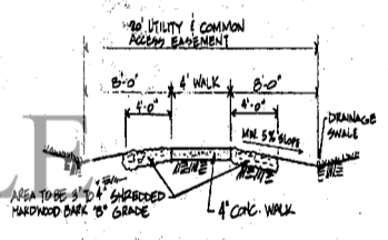
WALK DETAIL NO SCALE
