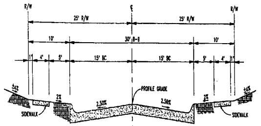
TYPICAL STREET SECTION N/S
