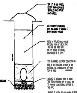
TRENCH DETAIL 1/4"=1'-0"
