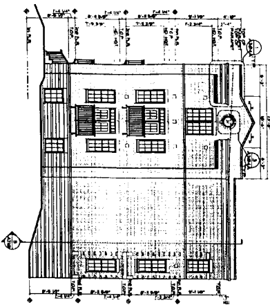
BUILDING V. RIGHT SIDE ELEVATION
