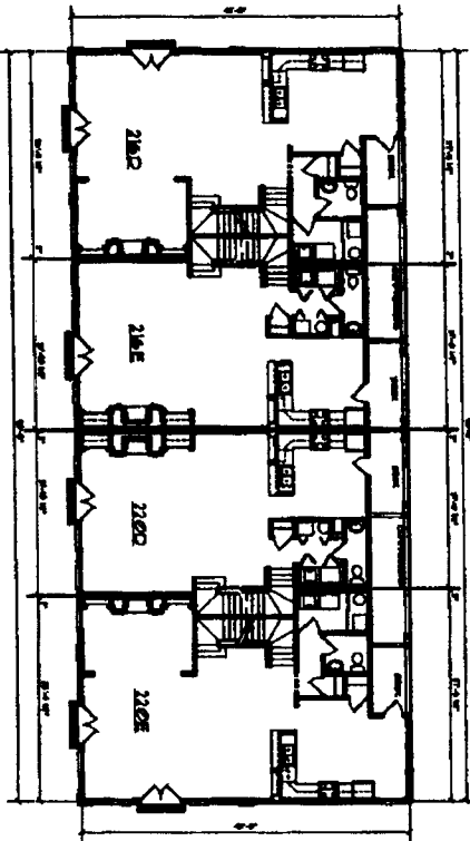
BUILDING 4 - 3RD FLOOR
