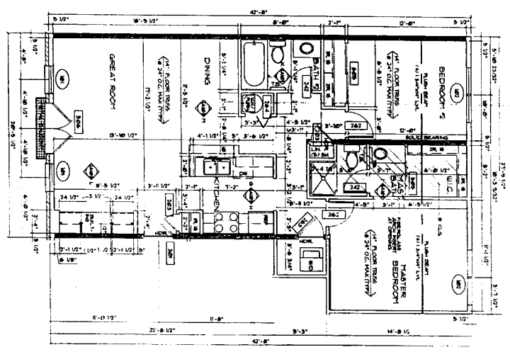
"THE BAILEY" 942 sq. ft. SCALE: 1/4" = 1'-0" REVERSE HAND
