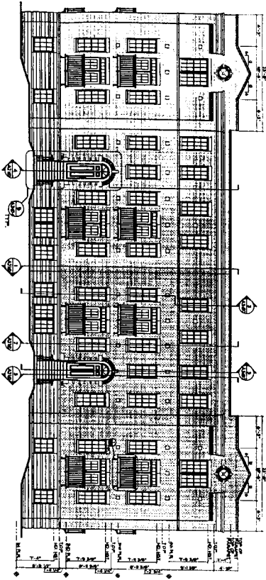
BUILDING III FRONT ELEVATION
