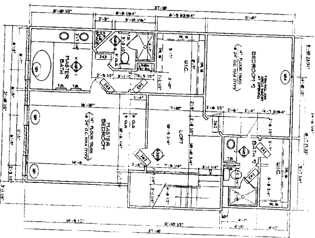
FOURTH FLOOR PLAN 780 SQ. FT.
