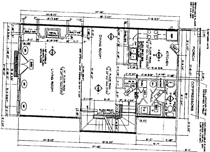
THIRD FLOOR PLAN 844 SQ. FT.
