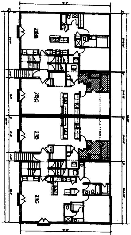
BUILDING 2 - 2ND FLOOR
