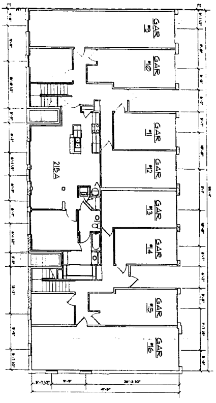
BUILDING 2 - 1ST FLOOR
