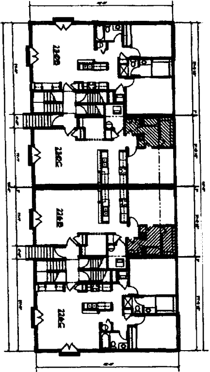
BUILDING 5 - 2ND FLOOR
