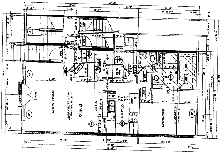
"THE CANTRELL" 812 sq. ft. SCALE: 1/4" = 1'-0" □ REVERSE HAND
