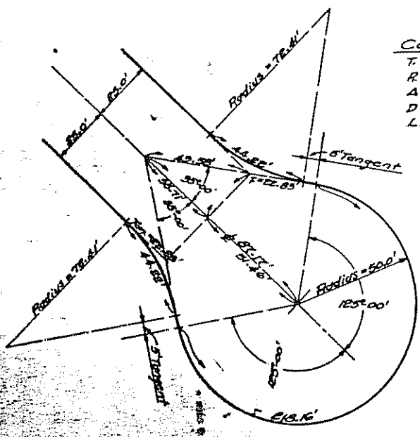
TYPICAL CUL-DE-SAC DETAIL Scale 1" = 30'-0"
