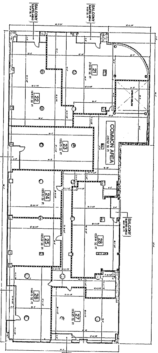
01 SECOND FLOOR PLAN FINISH FLOOR ELEVATION = 4'-11 1/2" CEILING ELEVATION = 4'-11 1/2" SCALE: 3/32" = 1'-0"
